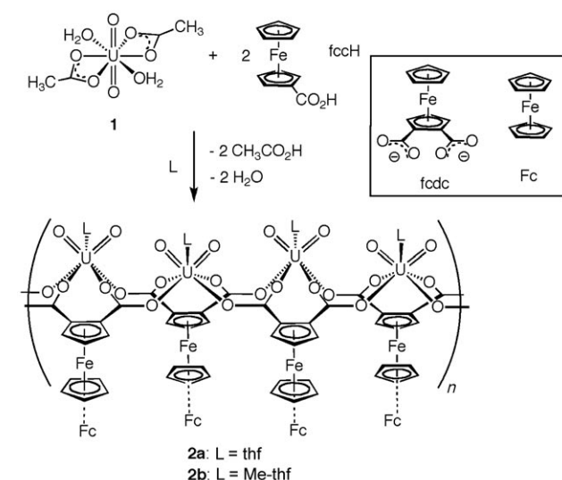
Scheme 1. Formation of the coordination polymers 2 .
